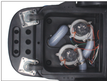
Removable access panel allows easy access to vacuum motors.
