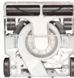
Easy Access to Belt, Brush Roll, Fan and Fan Chamber Without Tools! See Thru Cover Makes Inspection and Repair Easy!
