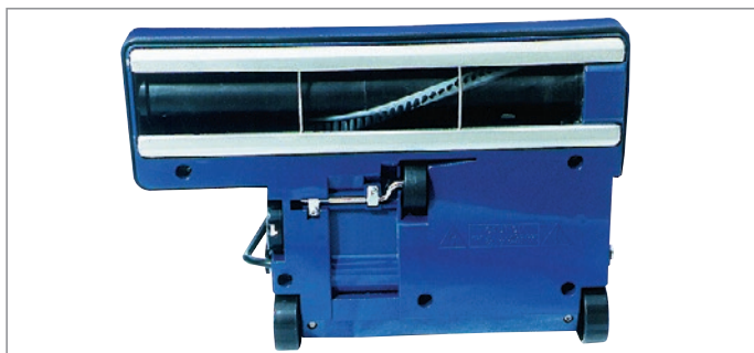
Replaceable single spiral brush strip does not require brush roll to be removed! Brush roll only operates with handle in operating position.
