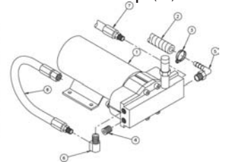
PFX1300 High Pressure Pump (14)
